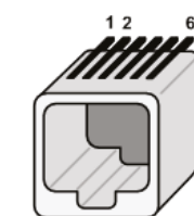
Metering System RJ12 female socket
